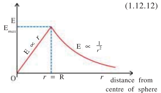
Figure 1.30 Electric Field of a Charged Sphere
